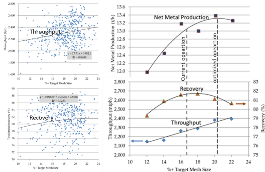
Figure 5: Throughput and recovery unfiltered (left), with data binning (right) with Net Metal Production (NMP) objective function per Equation 1.
