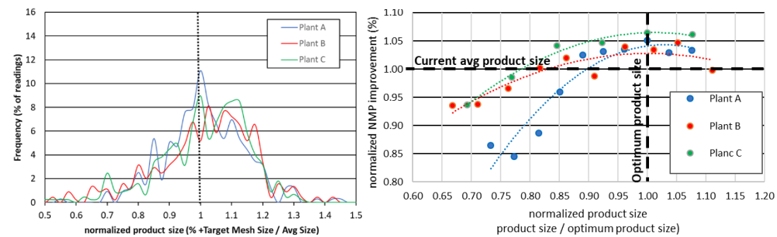
Figure 7: Normalized product size distribution without real-time size control (left); normalized NMP improvement.
