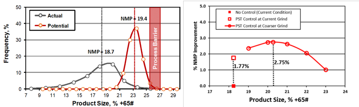
Figure 6: Actual and potential size distribution histograms and resultant NMPs (left) and associated potential percent NMP improvement (right).
