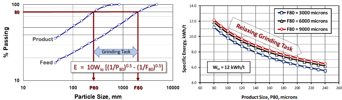
Figure 3: The ‘Grinding Task’ (left), and the effect of relaxing it (right).
