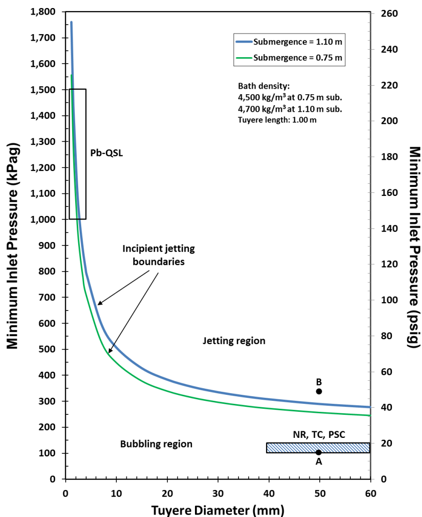
Figure 6: Sonic flow mapping: plots of the minimum tuyere back-pressure requirement as a function of tuyere diameter and submergence to achieve incipient jetting.
