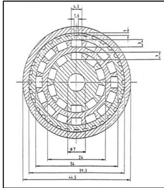
Figure 7: Cross-section of a QSL oxidation S-injector (reproduced from Arthur et al. , 1992).
