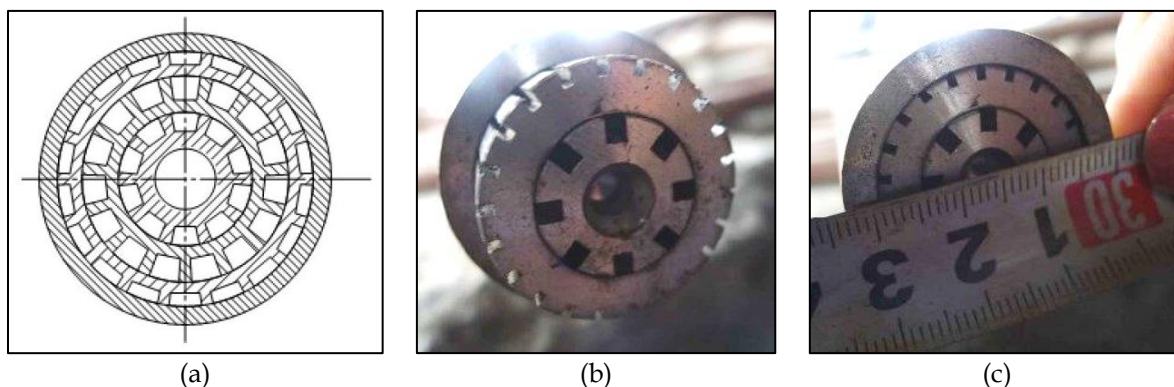
Figure 5: SKS/BBS shrouded injectors: (a) cross-section drawing from Hao et al. (2013); (b) and (c) photographs of SKS injector tip from ENFI presentation (2014).
