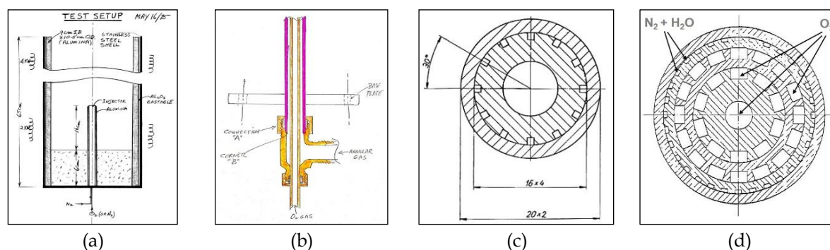
Figure 4: Evolution of the QSL oxygen injector: (a) bench scale, 1975; (b) pilot scale, 1977; (c) demonstration plant, 1981-86; and (d) commercial plant, 1989. (Air Liquide Canada Archives).
