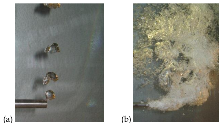
Figure 2: Still images of compressed air continuously injected into water: (a) bubbling regime with discrete gas bubbles; and (b) jetting regime with fully developed gas jet (Joël P.T. Kapusta Archives).
