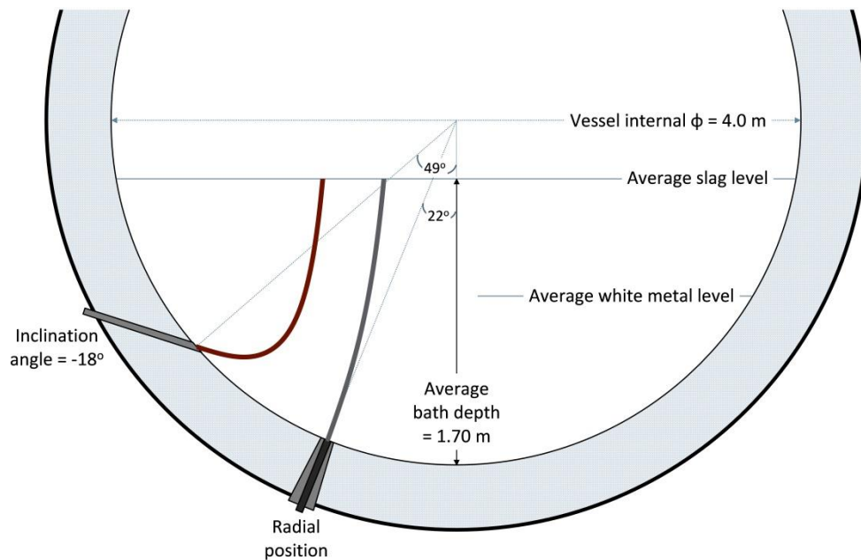
Figure 8: Scaled drawing of a copper bath smelting vessel with visualization of the calculated gas jet axis trajectories under jetting regime for side and bottom blowing (Kapusta, 2017).
