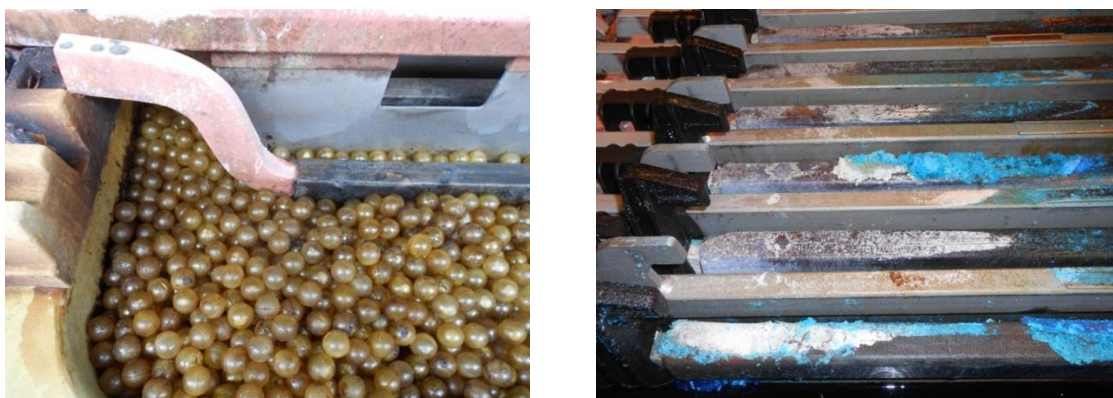
Figure 5. Corrosion of hanger bar due to immersion or seepage and corrosion of lead by \text{CuSO}_4 .
