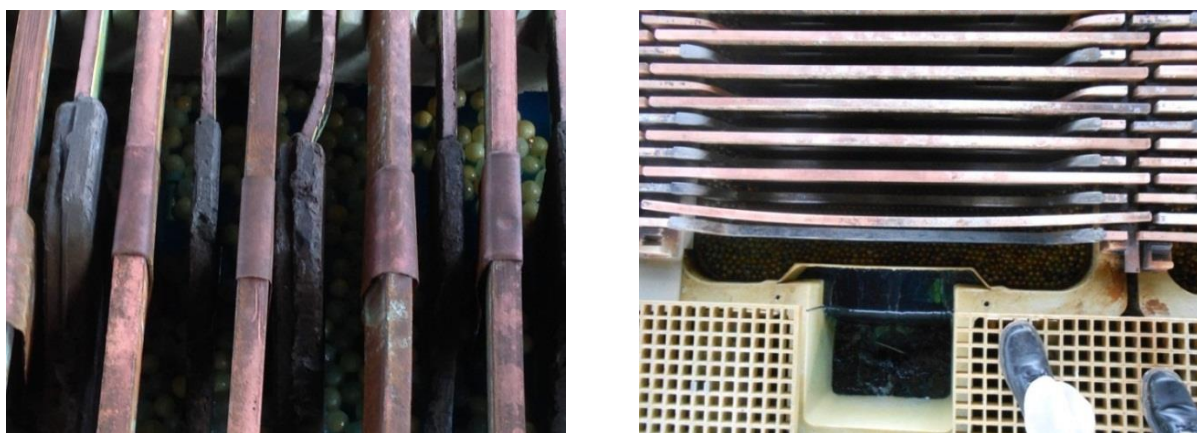
Figure 9. Uneven electrode spacing.
