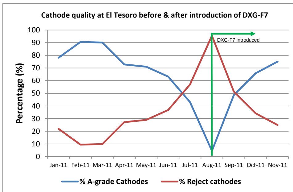
Figure 5. Turn around in cathode quality with the introduction of DXG-F7 at El Tesoro in August 2011.
