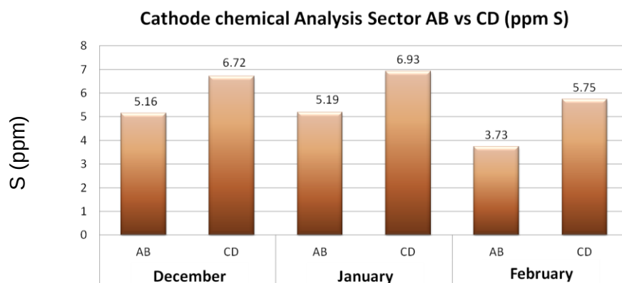
Figure 3. Effect of DXG-F7 on cathode sulphur content at Barrick's Zaldivar EW plant. DXG-F7 added to sector AB; guar added to sector CD; both sectors operated under the same current density and with the same electrolyte.
