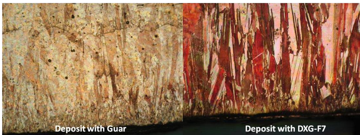
Figure 2. Cross sectional image of growth pattern of copper deposits with guar compared with that using DXG-F7 at Zaldivar, Chile (100x magnification). Current density 330 A/m 2 ; dosage 280 g/t; harvest cycle 5 days.
