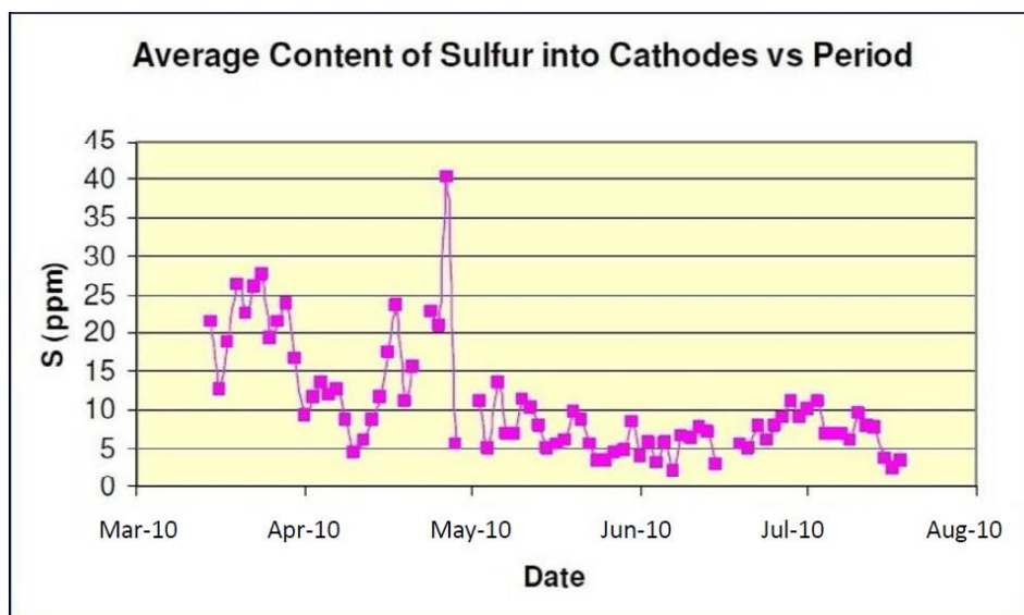
Figure 6. Reduction in sulphur levels in the copper cathodes at Los Bronces following introduction of DXG-F7 in April 2010.
