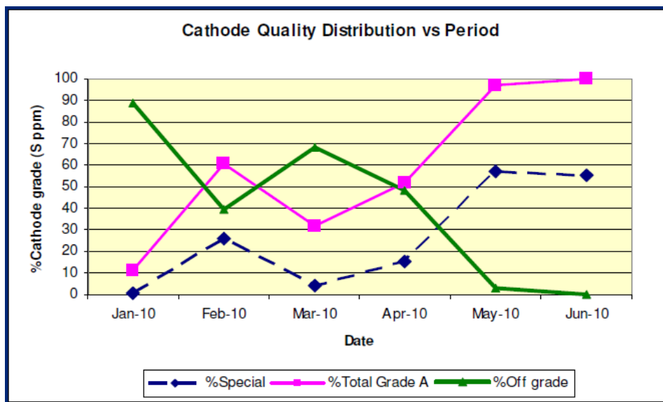
Figure 7. Improvement in copper quality at Los Bronces, following introduction of DXG-F7 in April 2010. ("Special Grade" is an in-house designator for cathodes of better quality than A-Grade.)
