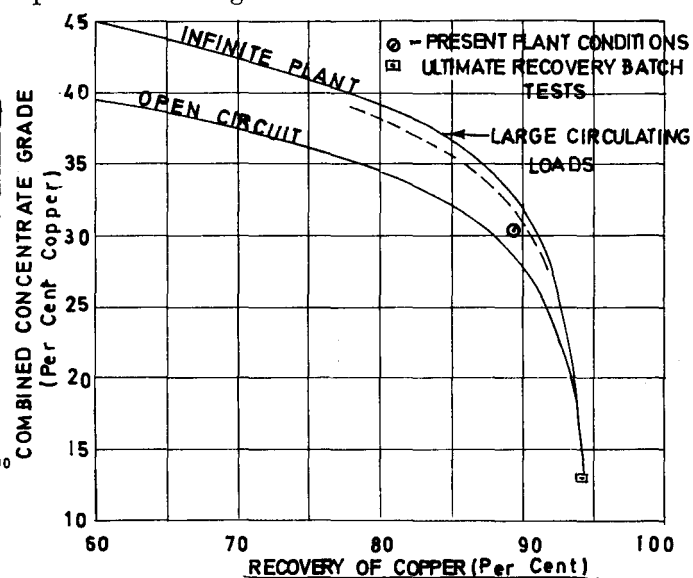
Fig. 5—Calculated grade-recovery curves
