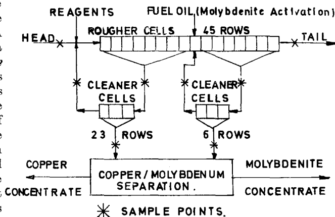
Fig. 1—Flow diagram of the primary separation in the Arthur Concentrator
