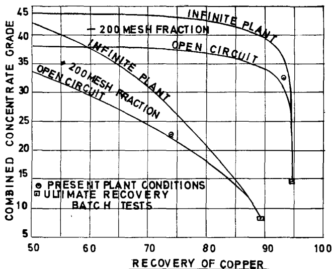
Fig. 6—Calculated grade-recovery curves for coarse and fine fractions
