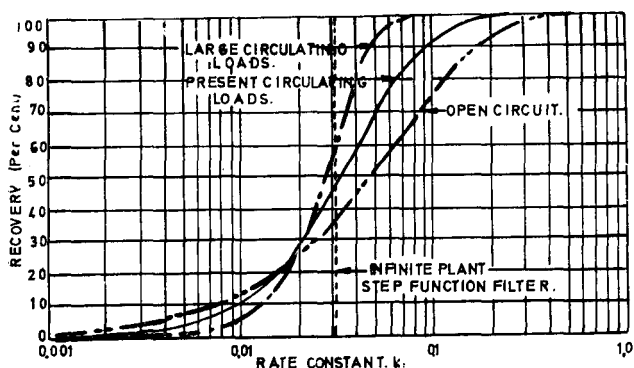
Fig. 4—Plant recovery of individual rate components for a constant grade of combined concentrate
