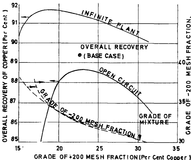
Fig. 7—Overall recovery of copper with separate circuits for coarse and fine fractions
