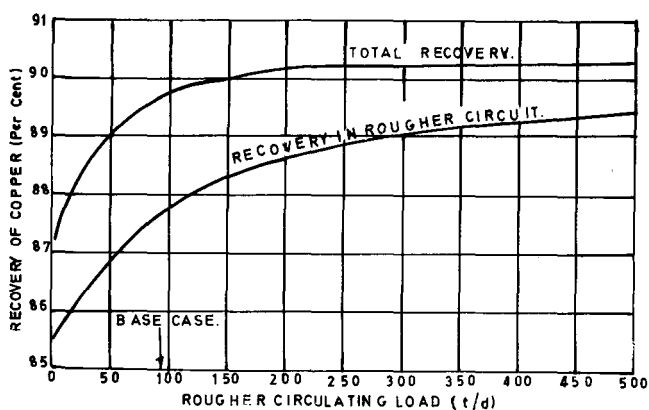
Fig. 3—Effect of circulating loads on recovery at constant grade of product (Scavenger circulating load proportional to rougher circulating load)
