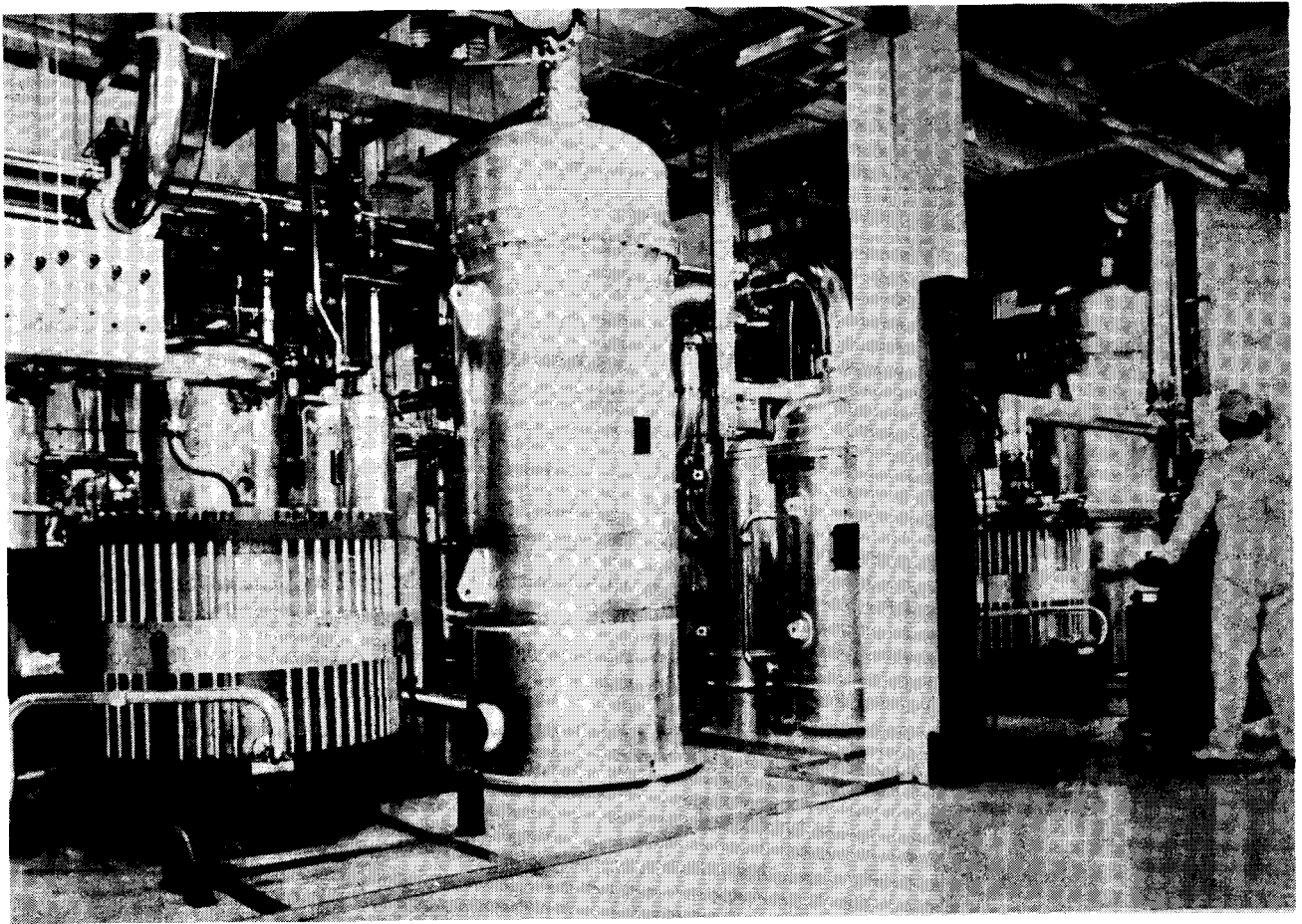
One of the stages of Ucor's uranium-enrichment plant
