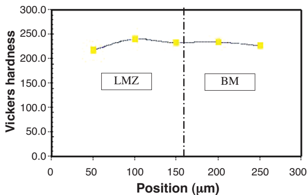
Figure 6—Microhardness across the transverse section of the sample submitted to laser surface melting
