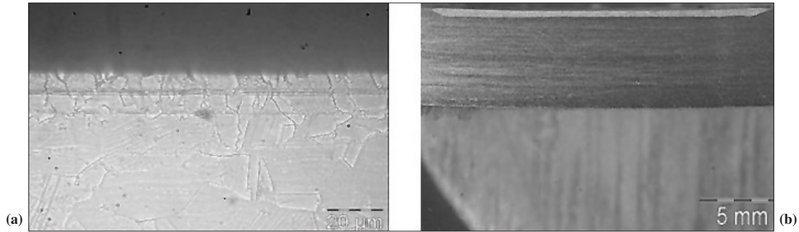
Figure 4—(a) Cross-sectional view of sample treated at 2.5 kW travelling at 10 mm/s, (b) Melt pool geometry at the same parameters as 4(a)
