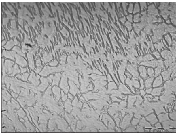
Figure 5—Microstructure of a laser-melted sample at 1000X
