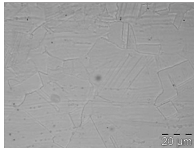
Figure 2—Microstructure of the starting material showing austenite grains and twin bands
