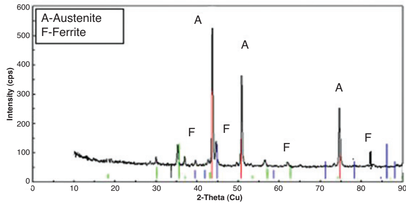
Figure 7—X-ray diffraction spectrum of a laser treated 304 SS
