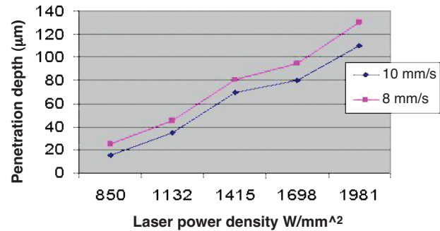
Figure 1—Relationship between laser power density and penetration depth
