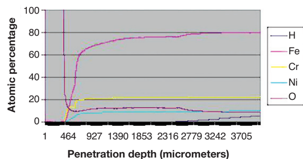
Figure 10—Glow discharge optical emission spectroscopy
