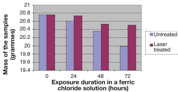
Figure 9—The tendency to lose mass of the untreated and laser treated samples
