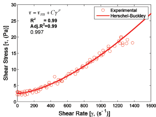
Figure 6—Herschel-Buckley model fit to d_{50} - 90 microns sand at C_v = 40\% (Model parameters: \tau_{HB} = 2.574 , C = 2.66 \times 10^{-4} and P = 1.55 )
