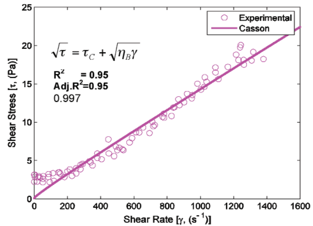
Figure 8—Casson model fit to d_{50} - 90 microns sand at C_v = 40\% (Model parameters: \tau_C = 0.183 and \eta_B = 0.013 )
