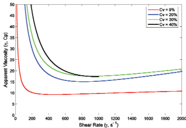
Figure 14—Apparent viscosity of d_{50} - 300 microns sand as a function of shear rate
