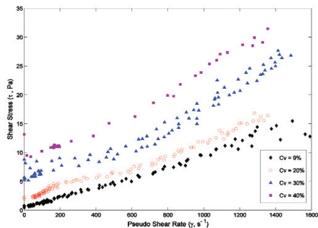
Figure 5—Rheograms for the d_{50} - 300 \mu\text{m} sand at different solids concentrations
