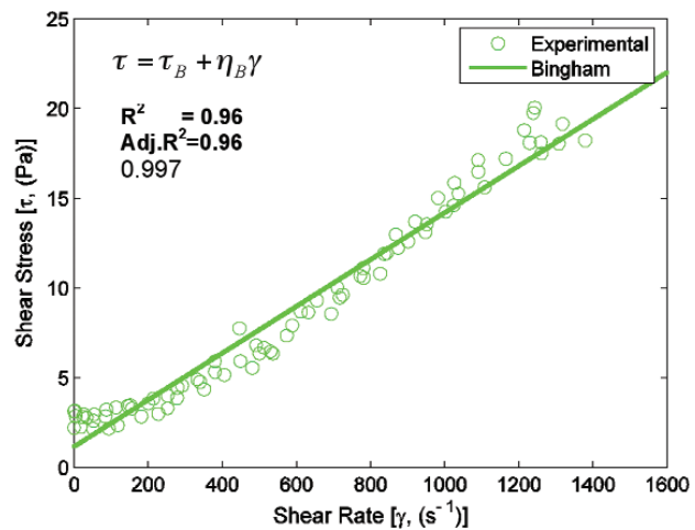
Figure 9—Bingham model fit to d_{50} - 90 microns sand at C_v = 40\% (Model parameters: \tau_B = 1.147 and \eta_B = 0.013 )
