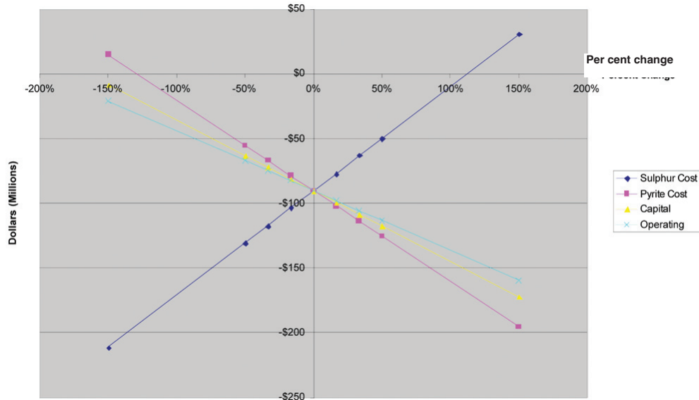
Figure 1—Sensitivity analysis—NPV (10%)
