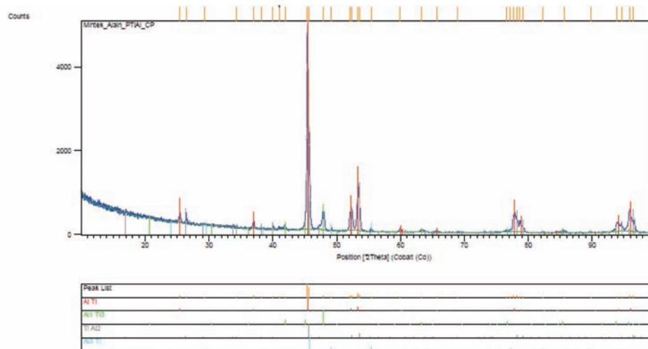
Figure 1—XRD pattern of commercial TiAl powder
