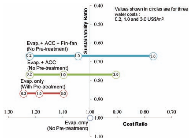
Figure 7—Hatch 4Q Analyses for water cost sensitivity
