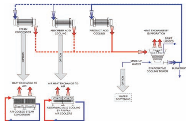
Figure 5—Water saving options schematic
