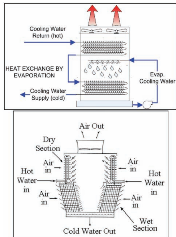
Figure 3—Hybrid cooler examples (after EPRI, 2002)
