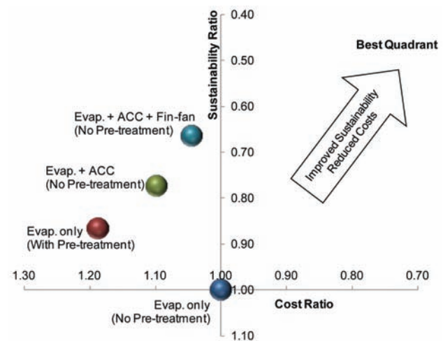
Figure 6—Hatch 4Q Analyses (average fresh water and power cost)
