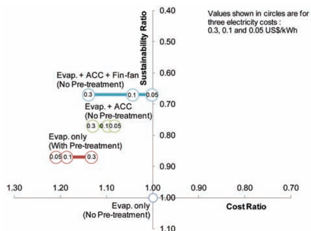
Figure 8—Hatch 4Q Analyses for electricity cost sensitivity
