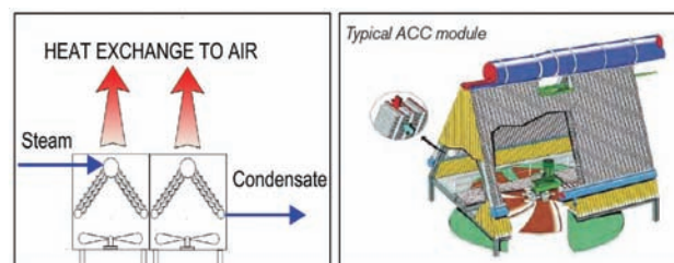
Figure 1 – Schematic of an ACC (SPX, 2012)
