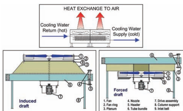
Figure 2—Fin-fan cooler (Wilson, 2011)
