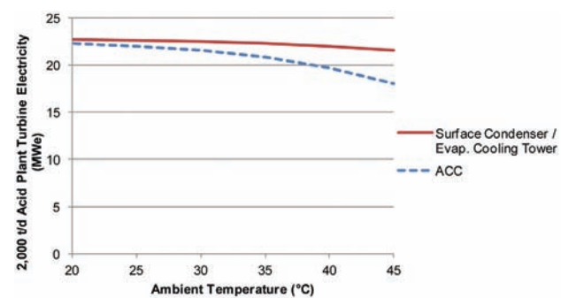
Figure 4—Impact of ambient temperature on turbine electricity generation
