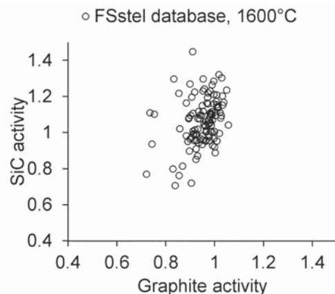
Figure 4—Activity of SiC (solid SiC as reference state) and activity of C (solid graphite as reference state) in Mn-Fe-Si-C metals at 1600°C, calculated with FactSage 6.4 (FSstel database) for the daily average tapped metal compositions. (Precipitation of solids suppressed)
