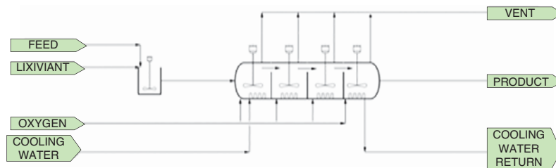
Figure 1—Base case circuit for pressure leaching
