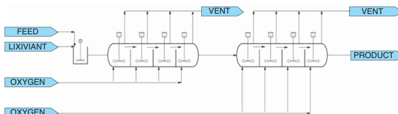
Figure 3—Series circuit for pressure leaching
