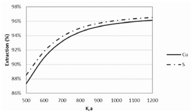
Figure 9—Effect of k_L a on overall conversions of copper and sulphur for the base case
