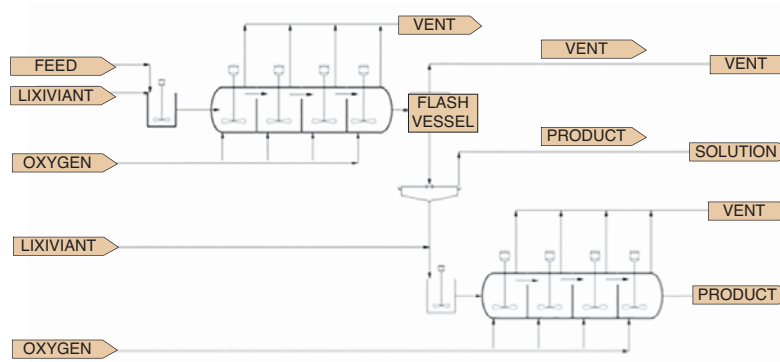
Figure 4—Series circuit with interstage thickening for pressure leaching
