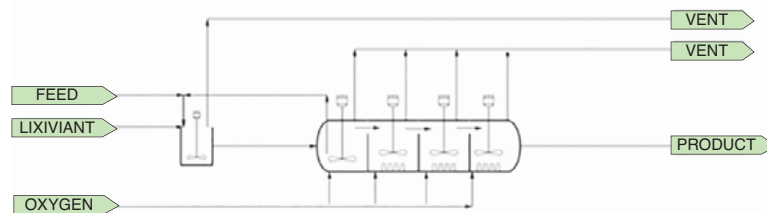
Figure 6—Flash recycling from the first compartment of an autoclave
