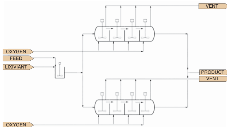
Figure 2—Parallel circuit for pressure leaching
