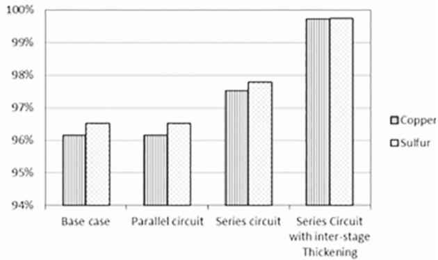
Figure 10—Overall extractions of copper and sulphur for all circuit options
