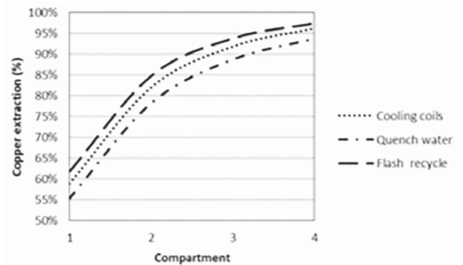
Figure 11—Overall copper extraction in each autoclave compartment for different heat removal options
