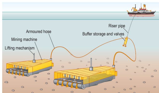
Figure 6—Industrial need for subsea crawler by Lehmköster (2022a)
